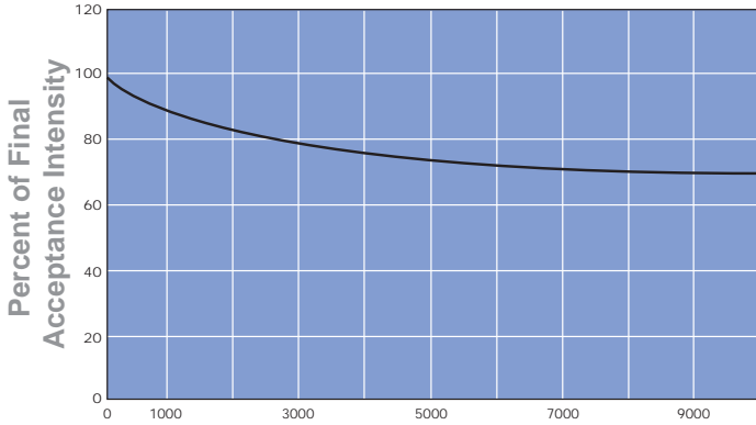
10K Zinc Lamp Typical Life Curve
