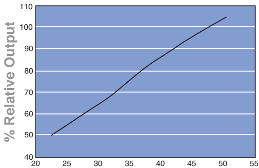
Light Output vs. Current
